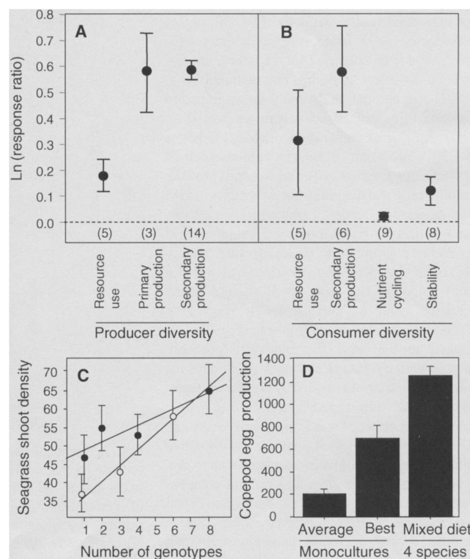
Fig. 1. Marine biodiversity and ecosystem functioning in controlled experiments. Shown are response ratios [\ln(\text{high}/\text{low diversity}) \pm 95\% \text{ confidence interval (CI)}] of ecosystem processes to experimental manipulations of species diversity of (A) primary producers (plants and algae), and (B) consumers (herbivores and predators). Increased diversity significantly enhanced all examined ecosystem functions ( 0.05 > P > 0.0001 ). The number of studies is given in parentheses. (C) Genetic diversity increased the recovery of seagrass ecosystems after overgrazing (solid circles) and climatic extremes (open circles). (D) Diet diversity enhanced reproductive capacity in zooplankton over both the average and best-performing monocultures.
