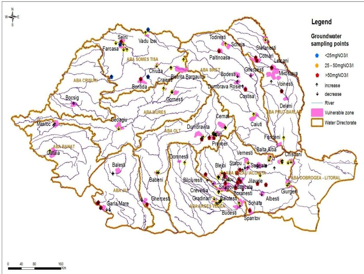
AVERAGE NITRATE CONCENTRATION IN GROUNDWATER SAMPLING POINTS(2012)
