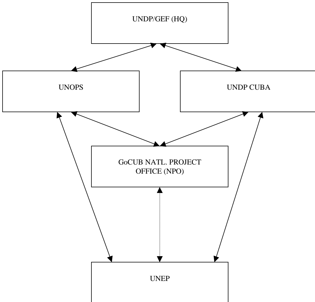
Figure 3: Project Organisation
